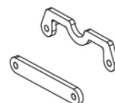
T4972/24 Support triangles arrière
